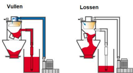
Vacuümhoppers werkings principe
