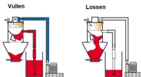
Vacuuhoppers werkings principe
